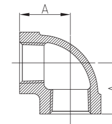
90° Reducing Elbow
