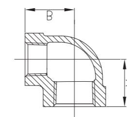
90° Reducing Elbow
