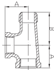
Service Tee
